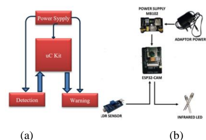
Figure 1. The proposed Low-Cost ESP32-CAM security system
